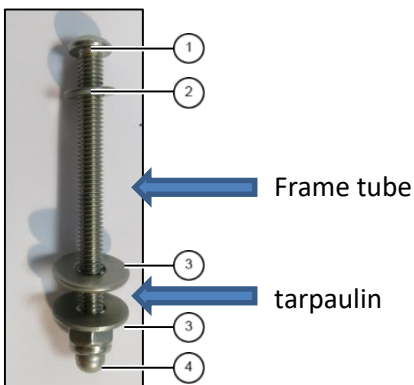
Fig. 1: bolt connection
